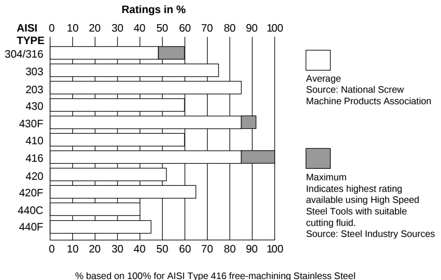
Figure 3 Comparative Machinability of Frequently Used Stainless Steels and Their Free-Machining Counterparts
